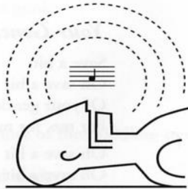
flute timbre
